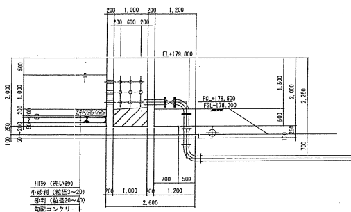
(天日乾燥床 (5))
