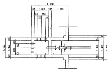
(天日乾燥床 (5))
