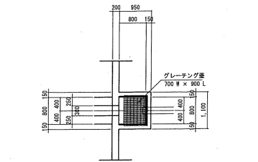
(天日乾燥床 (7))
