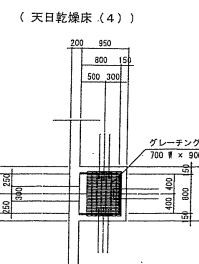
(天日乾燥床 (4))
