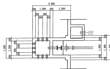
(天日乾燥床 (7))
