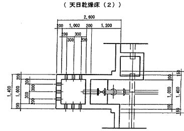
(天日乾燥床 (2))
