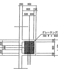
(天日乾燥床 (5))
