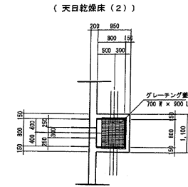
(天日乾燥床 (2))
