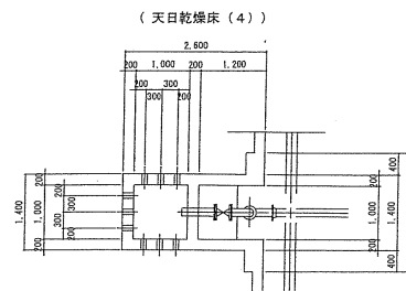
(天日乾燥床 (4))
